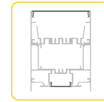
KN39 P37 max. 54mm
