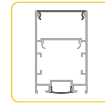
KN61 P40 max. 27mm
