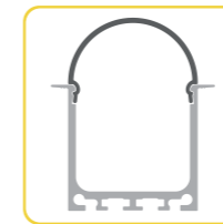
KN7-C13 P33 max. 17mm
