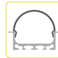
KN5-C13 P32 max. 18mm
