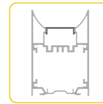
KN53 P39 max. 27mm
