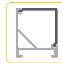
KM19 P42 max. 10mm
