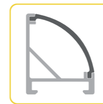
KM18 P42 max. 10mm
